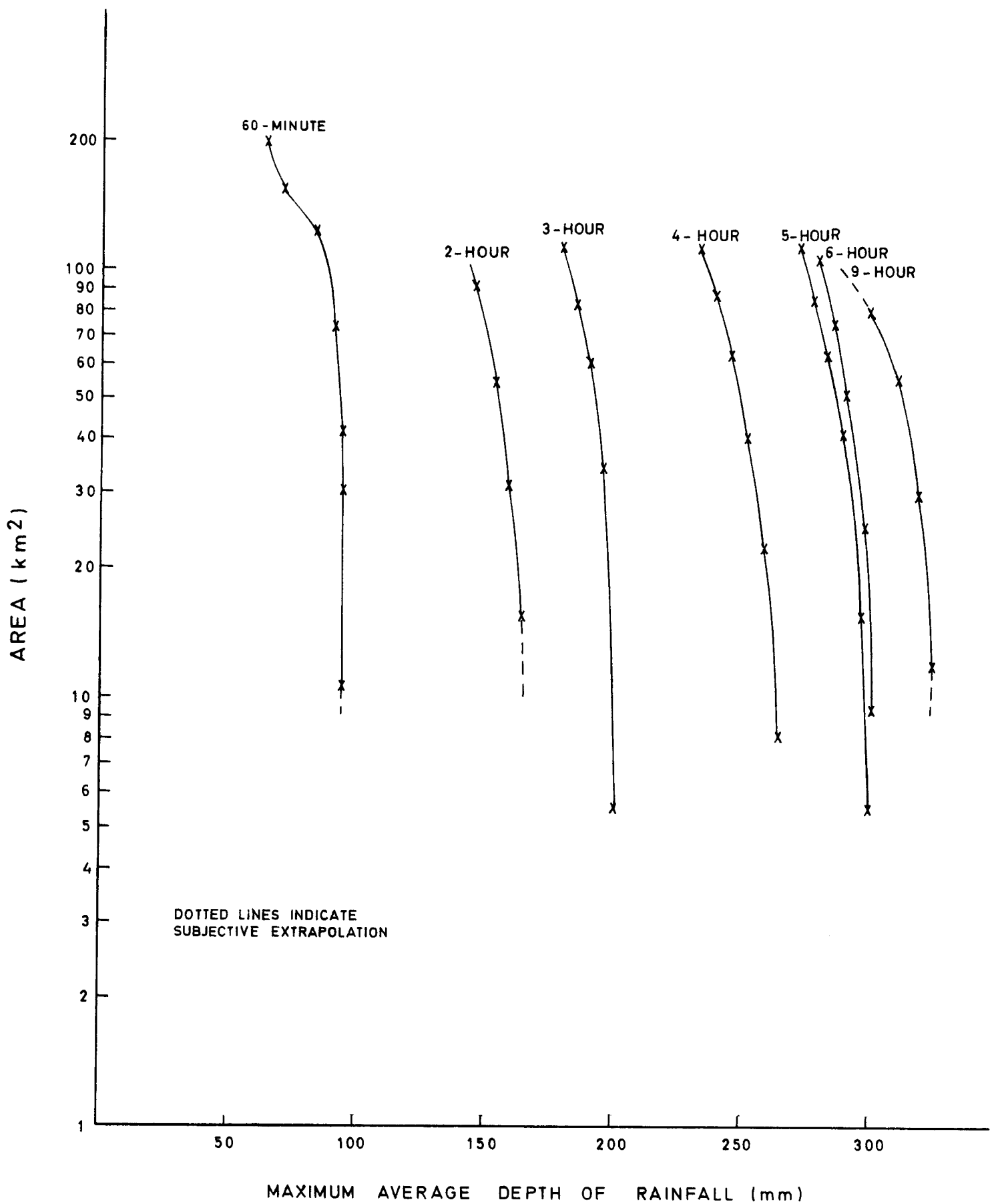
Fig.10 Depth-area-duration curves for the rainstorms on 17 June 1983
