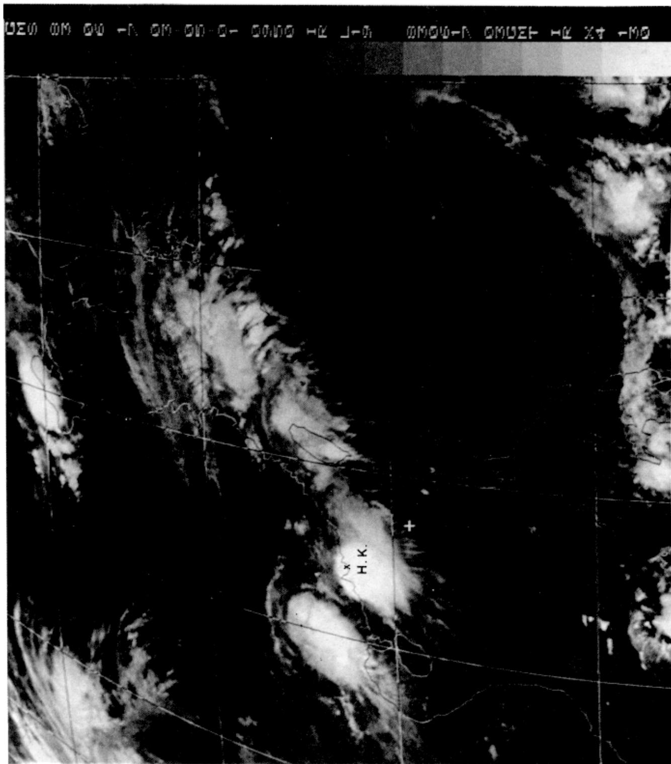
Plate 4. Infrared imagery taken at 11 a.m., 17 June 1983
