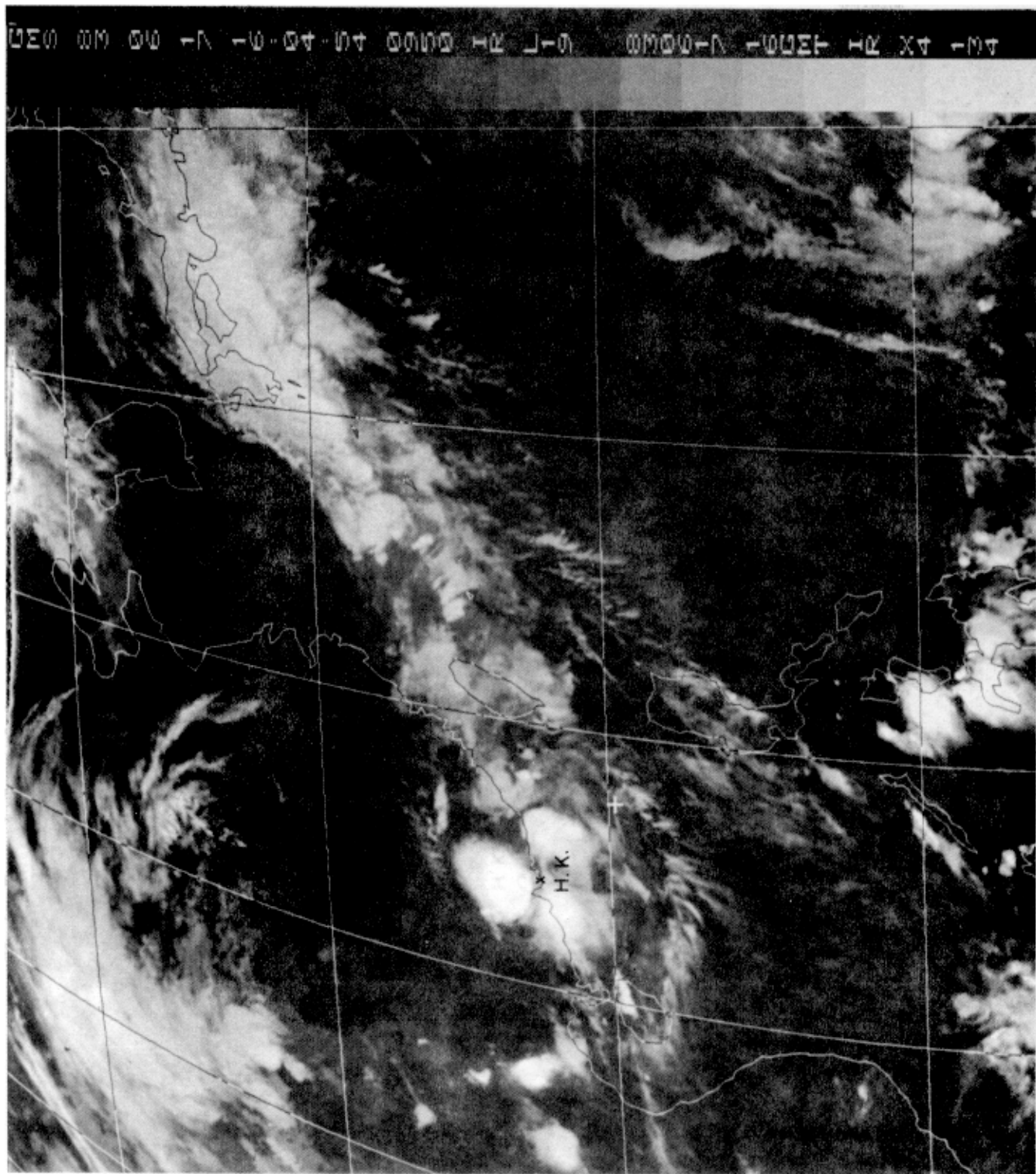
Plate 8. Infrared imagery taken at midnight, 17 June 1983
