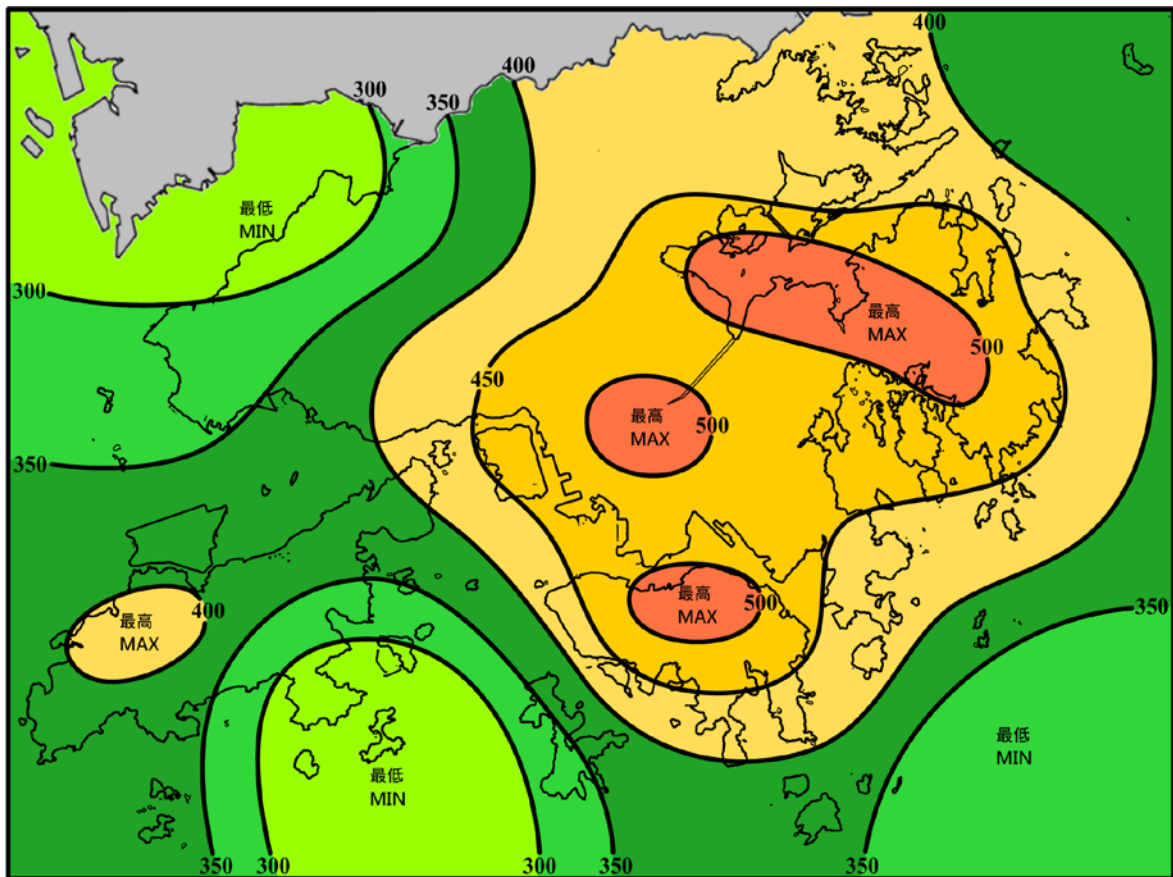
圖 11 (續) 二零一七年八月的雨量圖 (等雨量線單位為毫米) Figure 11 (cont'd) Rainfall Map for August 2017 (isohyets are in millimetres)
