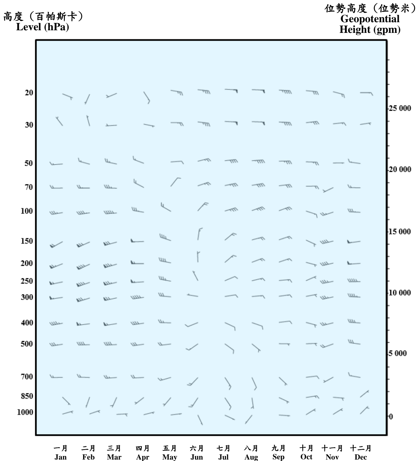
圖 13 各標準層於二零一七年協調世界時零時的月平均矢量風 Figure 13 Monthly Vector Mean Wind at Standard Levels at 00 UTC in 2017
