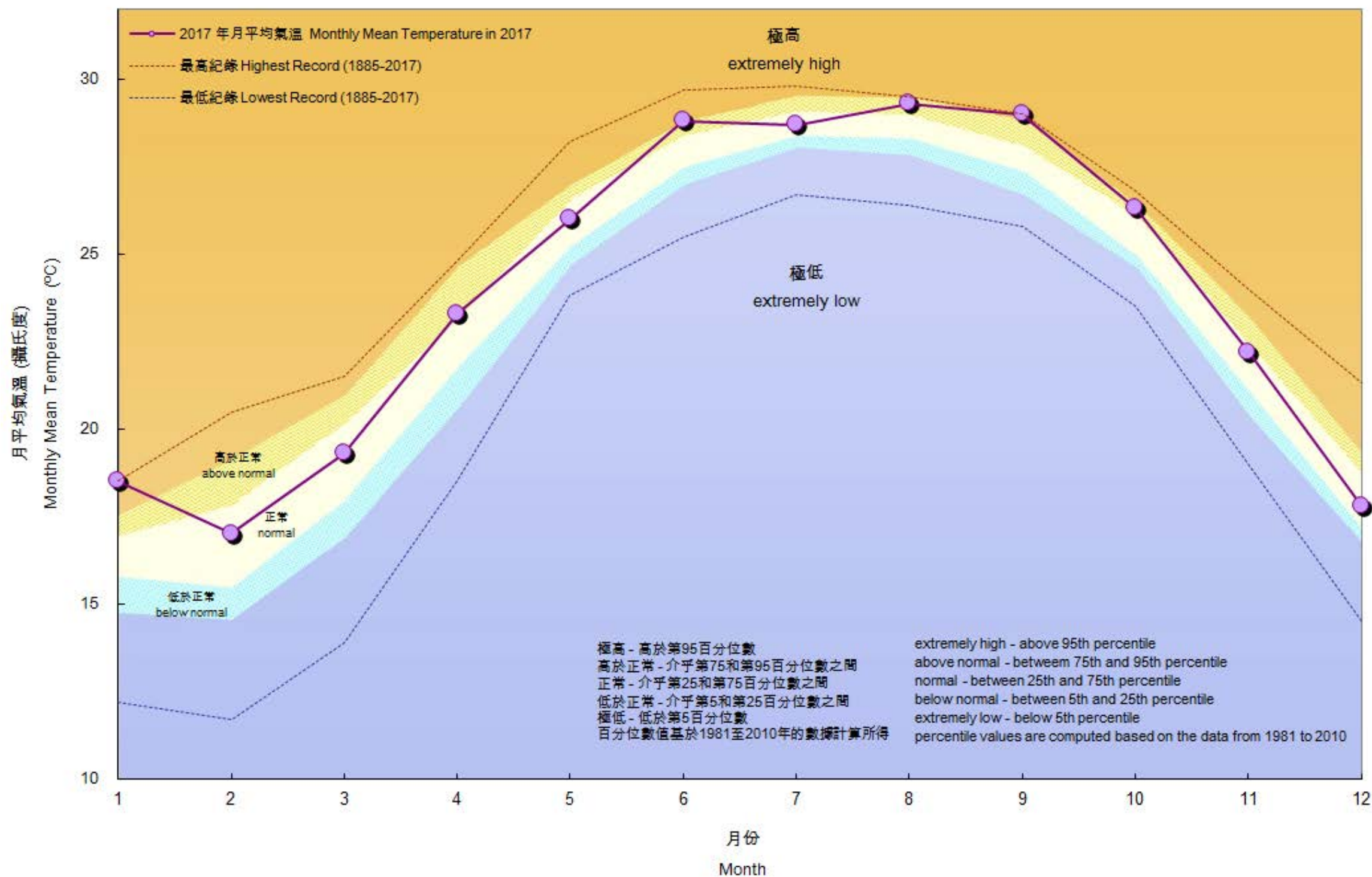
Figure 9 Monthly Mean Temperature at the Hong Kong Observatory in 2017
