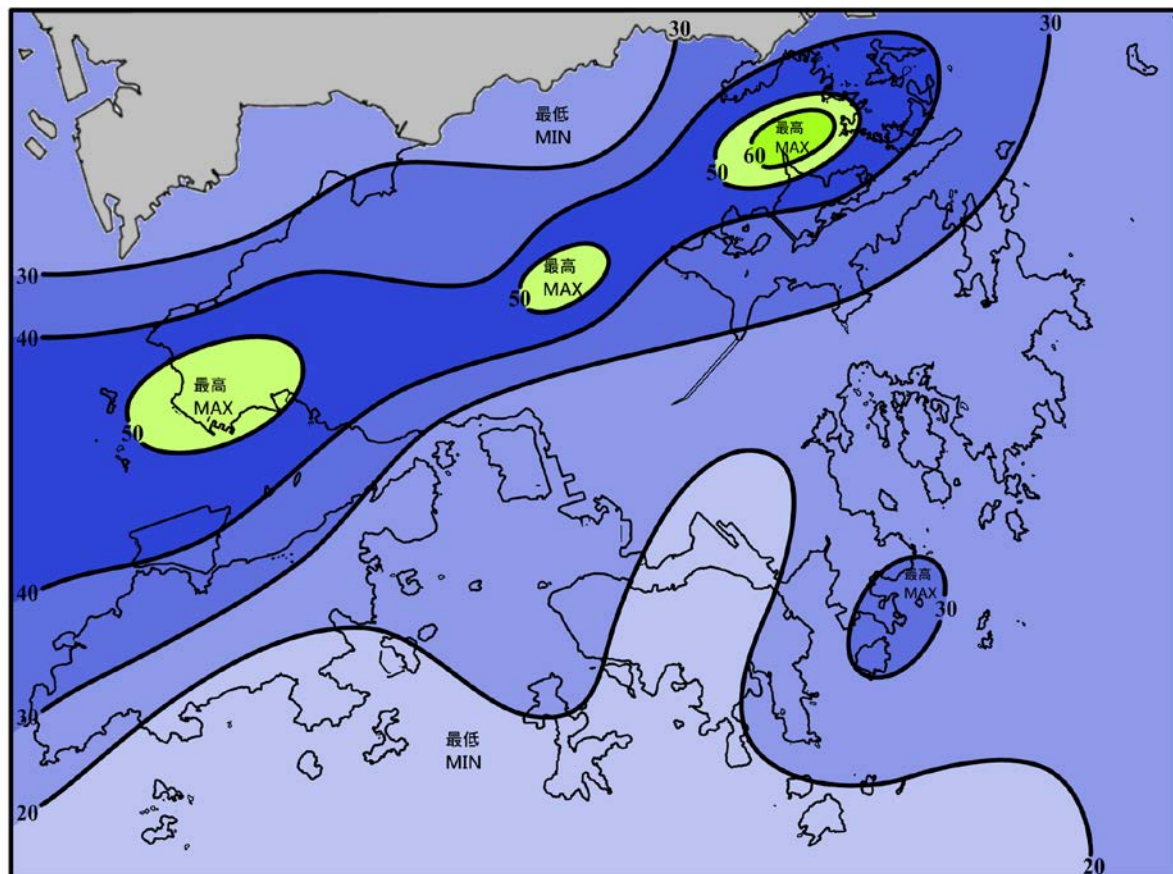
圖 11 (續) 二零一七年二月的雨量圖 (等雨量線單位為毫米) Figure 11 (cont'd) Rainfall Map for February 2017 (isohyets are in millimetres)
