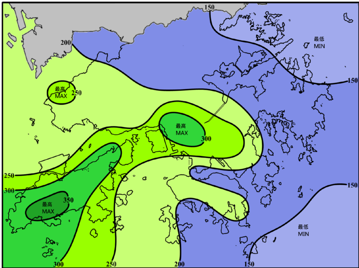
圖 11 (續) 二零一七年九月的雨量圖 (等雨量線單位為毫米) Figure 11 (cont'd) Rainfall Map for September 2017 (isohyets are in millimetres)
