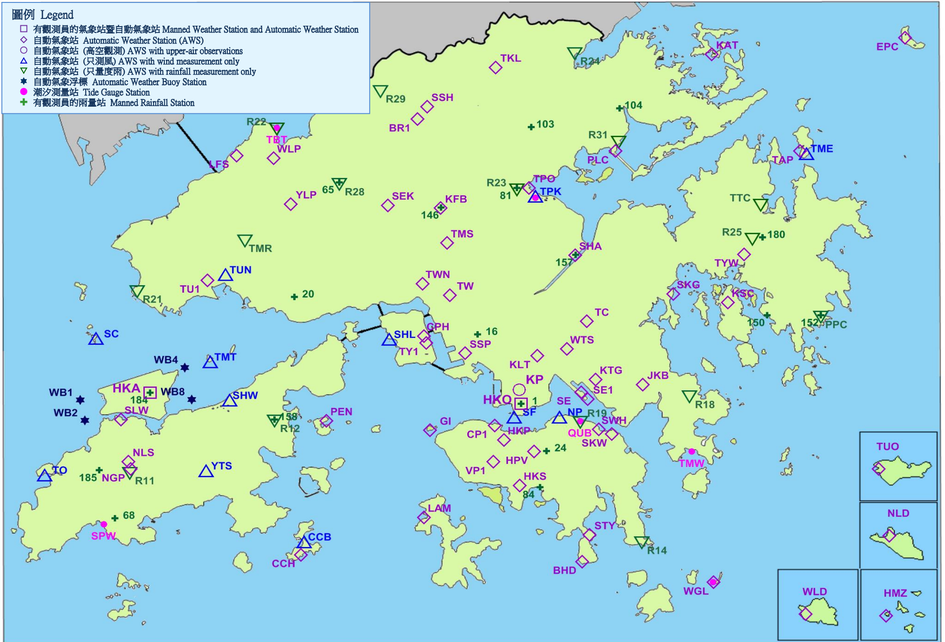
圖 1 氣象站、雨量站及潮汐測量站的位置圖 (二零一七年十二月三十一日) Figure 1 Locations of Weather Stations, Rainfall Stations and Tide Gauge Stations as at 31 December 2017.
