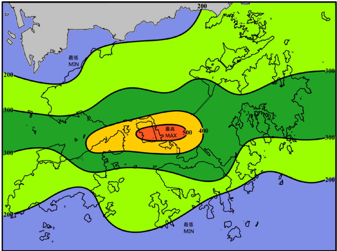
圖 11 (續) 二零一七年五月的雨量圖 (等雨量線單位為毫米) Figure 11 (cont'd) Rainfall Map for May 2017 (isohyets are in millimetres)
