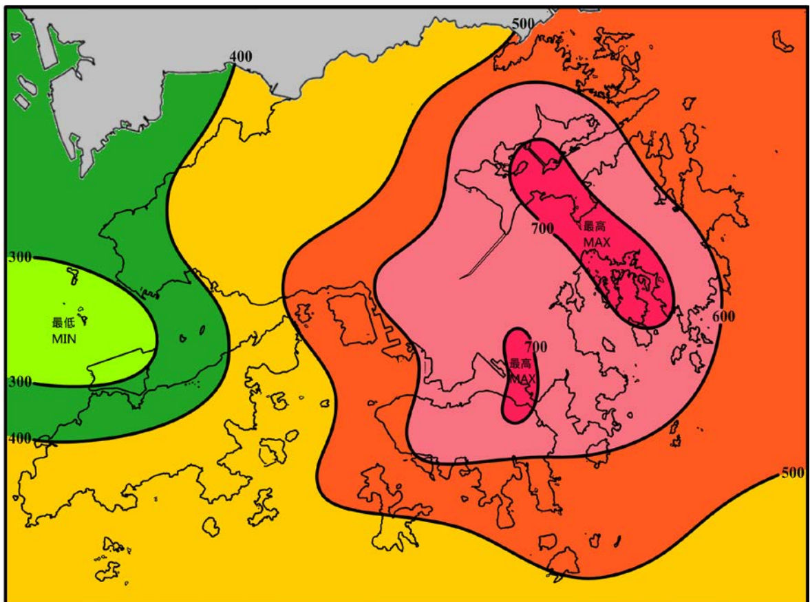
圖 11 (續) 二零一七年六月的雨量圖 (等雨量線單位為毫米) Figure 11 (cont'd) Rainfall Map for June 2017 (isohyets are in millimetres)
