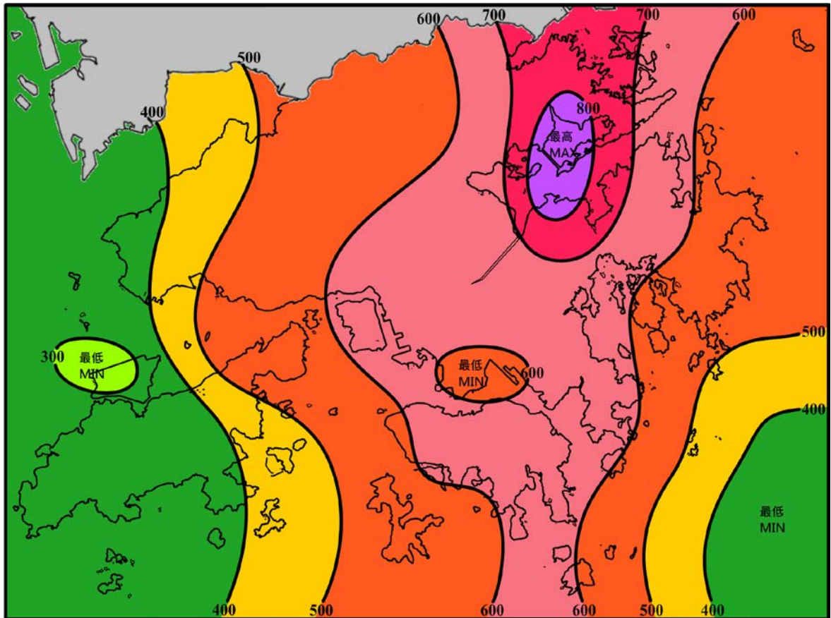
圖 11 (續) 二零一七年七月的雨量圖 (等雨量線單位為毫米) Figure 11 (cont'd) Rainfall Map for July 2017 (isohyets are in millimetres)
