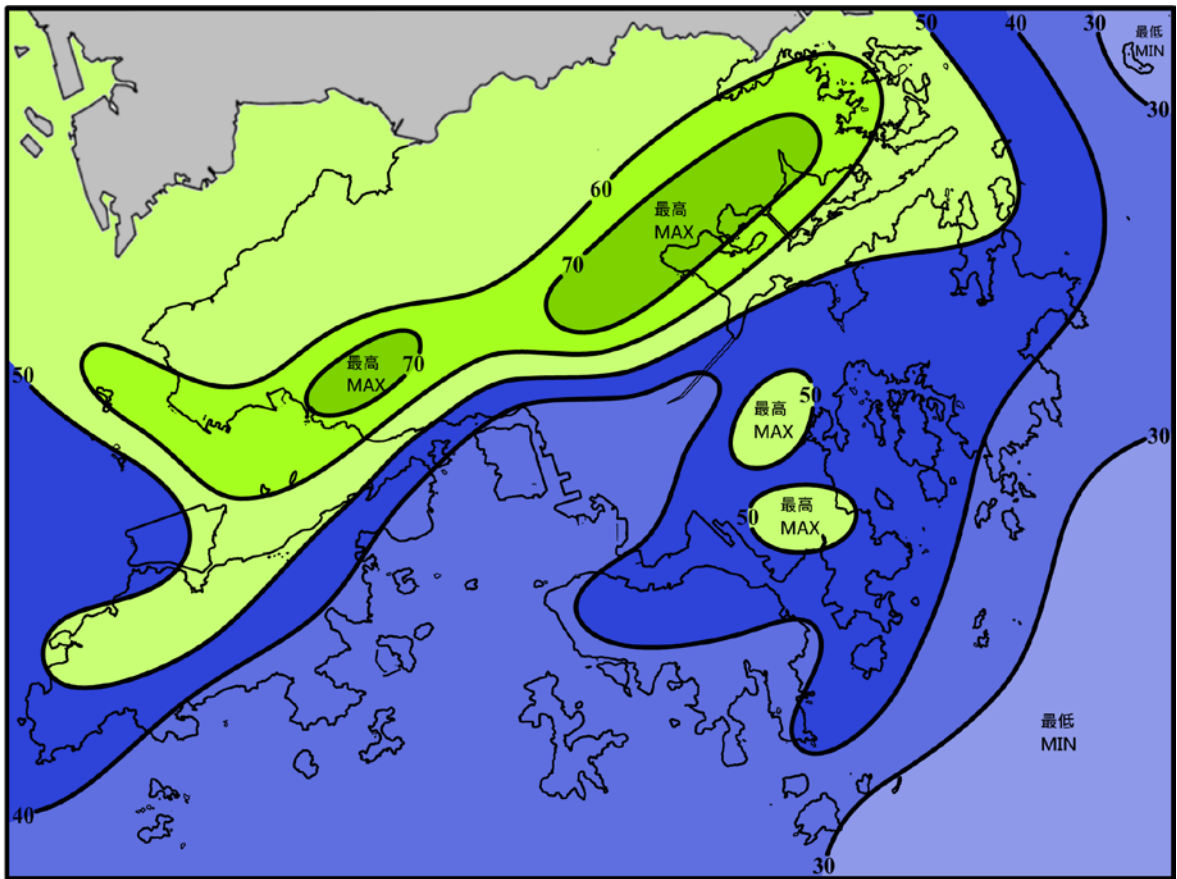
圖 11 (續) 二零一七年三月的雨量圖 (等雨量線單位為毫米) Figure 11 (cont'd) Rainfall Map for March 2017 (isohyets are in millimetres)
