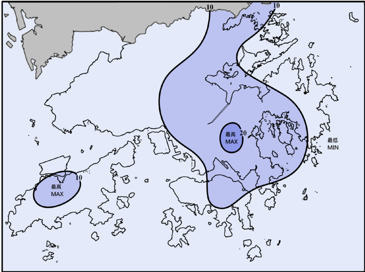
圖 11 二零一七年一月的雨量圖 (等雨量線單位為毫米) Figure 11 Rainfall Map for January 2017 (isohyets are in millimetres)
