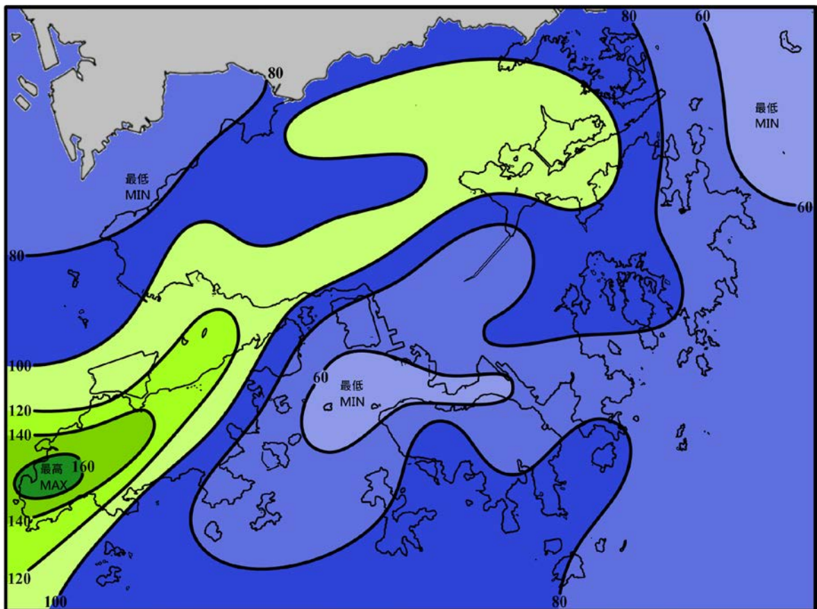
圖 11 (續) 二零一七年四月的雨量圖 (等雨量線單位為毫米) Figure 11 (cont'd) Rainfall Map for April 2017 (isohyets are in millimetres)
