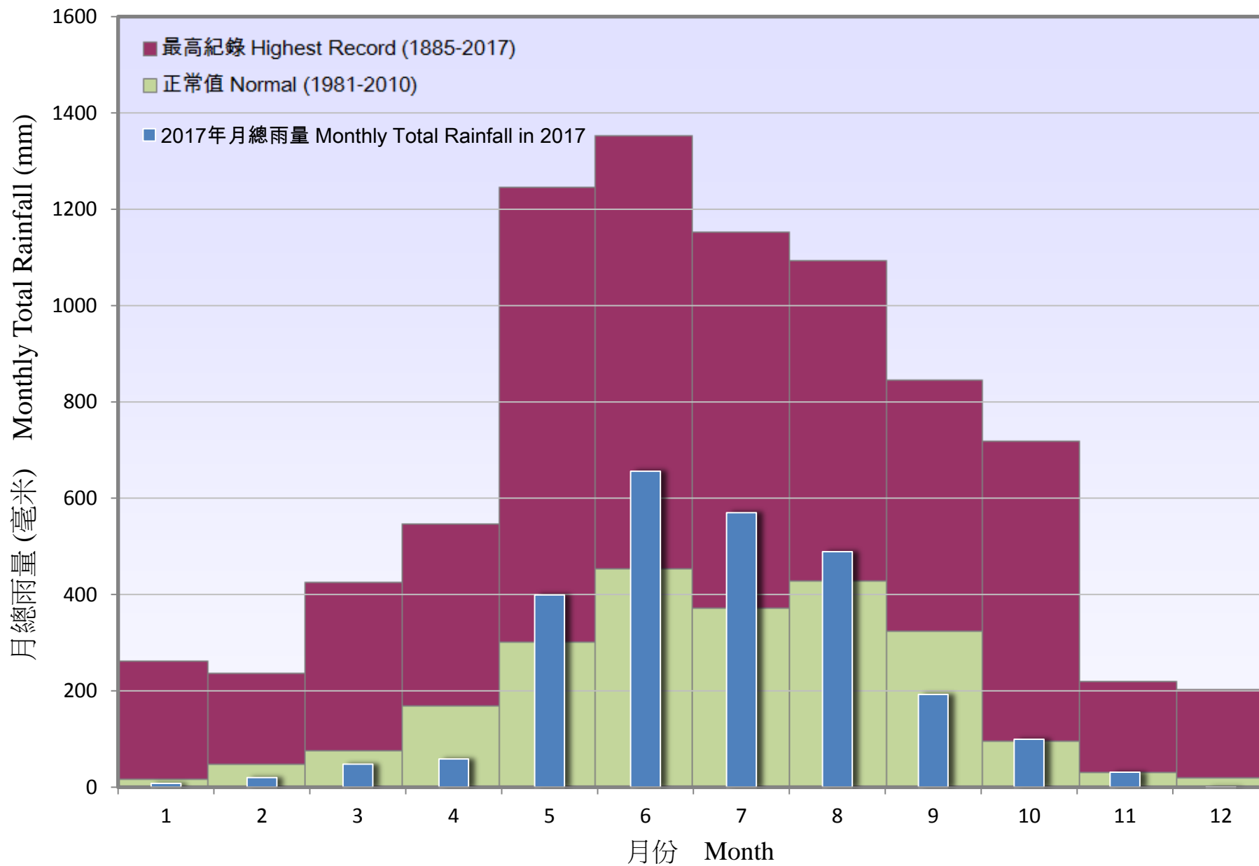
圖 10 天文台於二零一七年每月的總雨量 Figure 10 Monthly Total Rainfall at the Hong Kong Observatory in 2017
