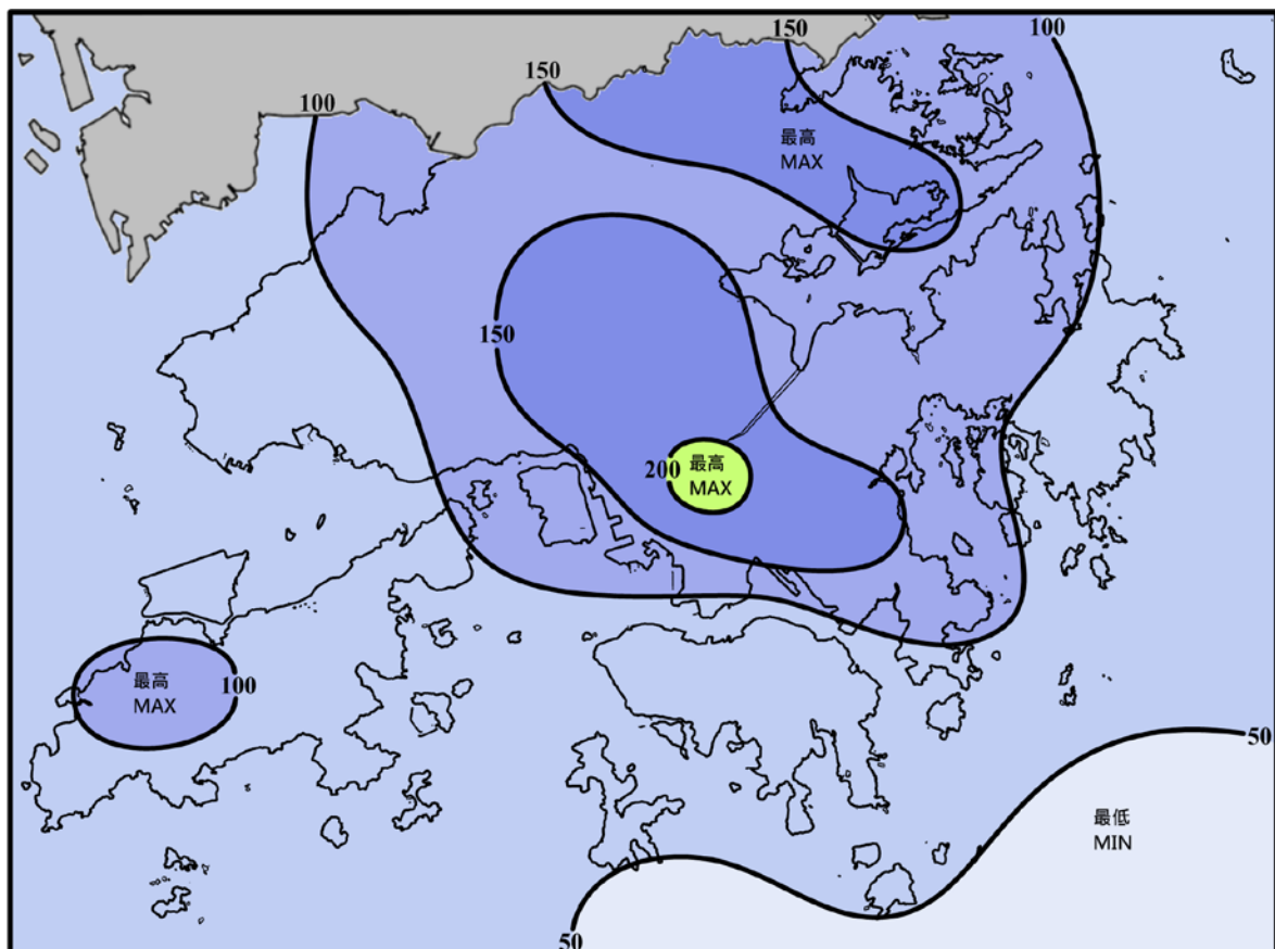
圖 11 (續) 二零一七年十月的雨量圖 (等雨量線單位為毫米) Figure 11 (cont'd) Rainfall Map for October 2017 (isohyets are in millimetres)
