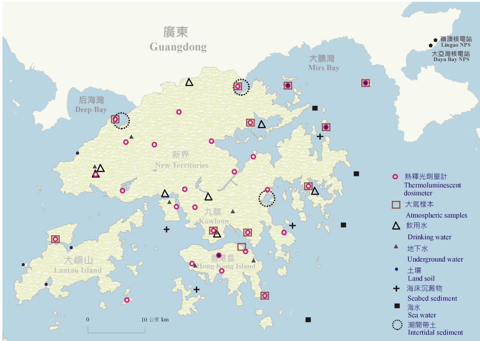
圖 3. 熱釋光劑量計網絡及二零一八年環境樣本收集點。 Figure 3. Thermoluminescent dosimeter network and locations for collection of environmental samples in 2018.
