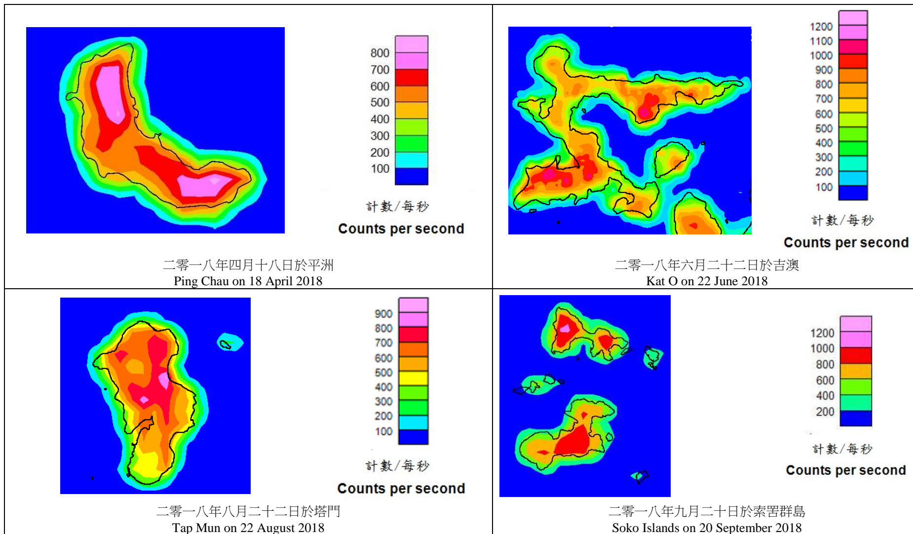
圖 4. 空中輻射監測系統在二零一八年分別於平洲、吉澳、塔門和索罟群島測量到的計數率(測量高度距離地面約一百米)。 Figure 4. Count rate over Ping Chau, Kat O, Tap Mun and Soko Islands respectively as measured by the Aerial Radiation Monitoring System in 2018 (at about 100 metres above the ground).
