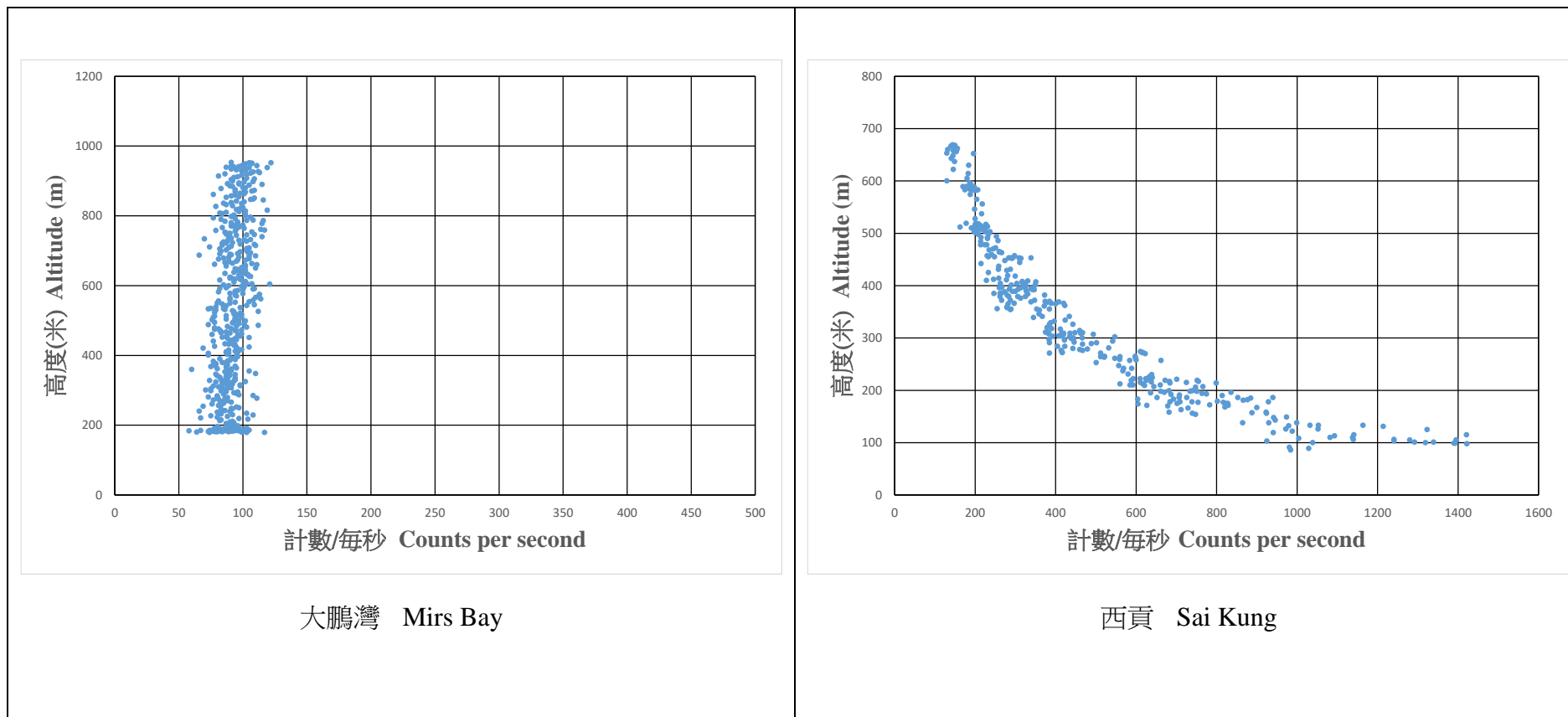
圖 5. 空中輻射監測系統在二零一八年七月十二日於大鵬灣海面及西貢上空測量到的計數率隨高度的變化。 Figure 5. Variation of count rate with altitude over Mirs Bay and Sai Kung area, as measured by the Aerial Radiation Monitoring System on 12 July 2018.
