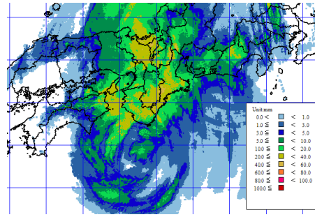
Figure 2. An example of R/A used in JMA: 17 UTC 15 Sep. 2013 (Typhoon MAN-YI)
