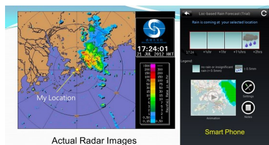
Figure 11. A comparison of the radar image with the location specific rainfall nowcast as shown on MyObservatory of HKO.
