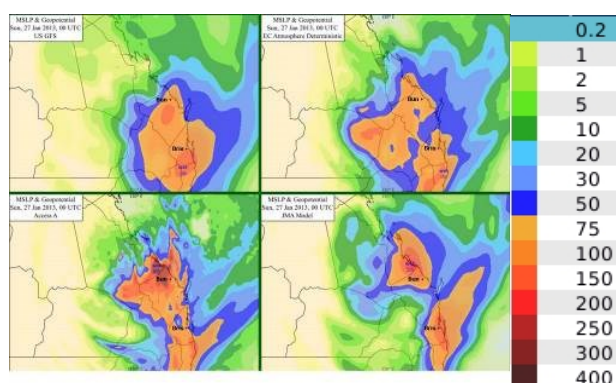
Figure 22. Deterministic NWP output for the 24 hours to 00 UTC on the 27 Jan 2013 (from 12 UTC runs on 25 Jan). The cities of Brisbane (Bris) and Bundaberg (Bun) are also shown.
