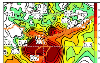
Figure 9. The 24-h extreme precipitation index forecast of Super Typhoon Rammasun (2014) as used by NMC/CMA.
