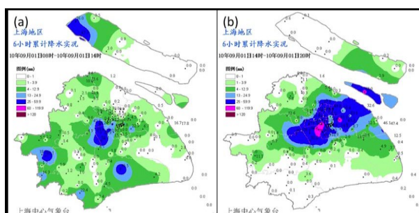
Figure 14. Rainfall in Shanghai during (a) 00 – 06 UTC and (b) 06 – 12 UTC on September 1, 2010 (adapted from Qi and Cao, 2013)
