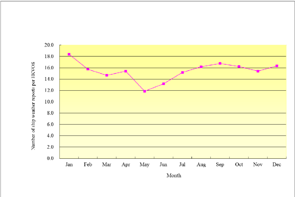
Number of ship weather reports per HKVOS in 2016
