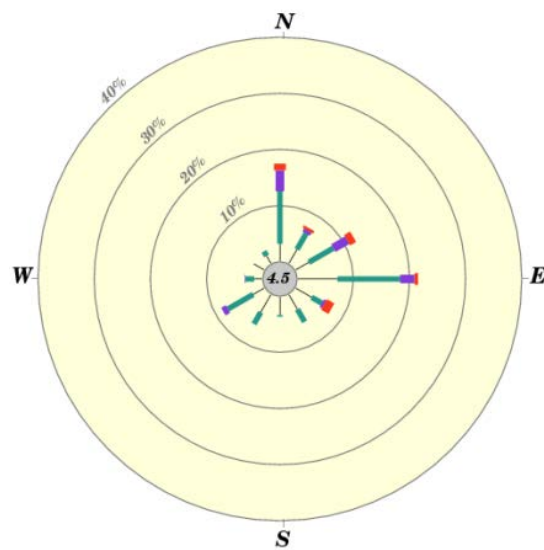
圖 7 (續) 橫瀾島於二零一八年每月的風玫瑰圖(七月至十二月) Figure 7 (cont'd) Monthly wind roses for Waglan Island in 2018 (July to December)
