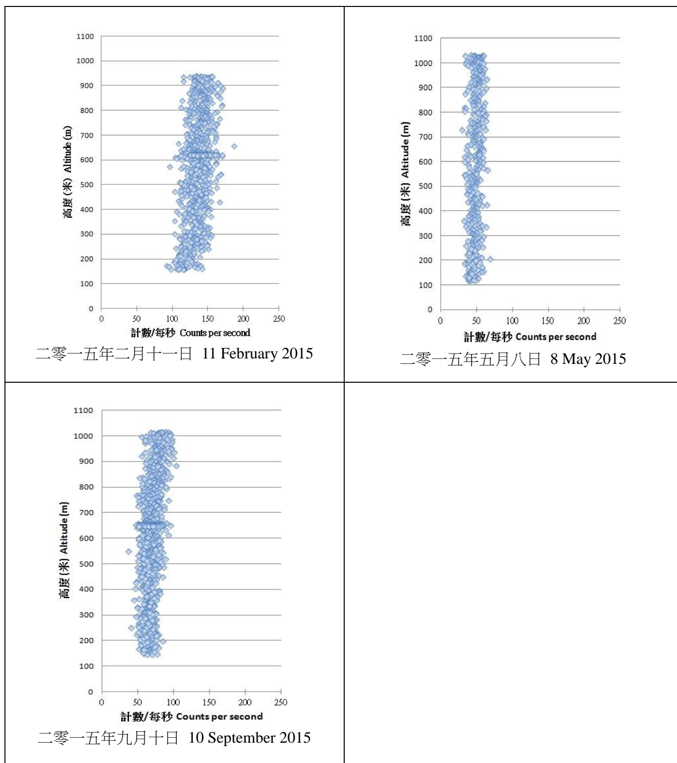
圖 4. 空中輻射監測系統在二零一五年於大鵬灣海面上空測量到的計數率隨高度的變化。 Figure 4. Variation of count rate with altitude at Mirs Bay, as measured by the Aerial Radiation Monitoring System in 2015.
