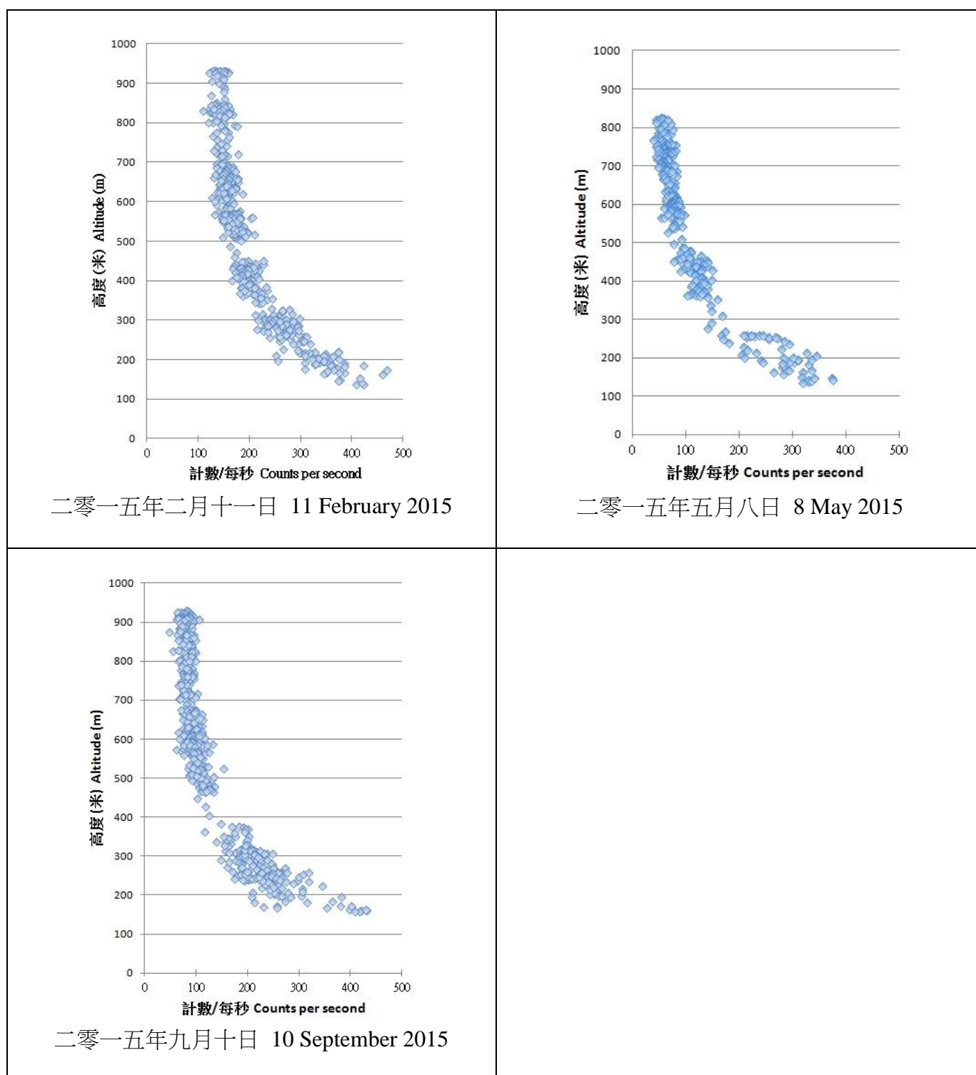
圖 5. 空中輻射監測系統在二零一五年於西貢上空測量到的計數率隨高度的變化。 Figure 5. Variation of count rate with altitude at Sai Kung, as measured by the Aerial Radiation Monitoring System in 2015.
