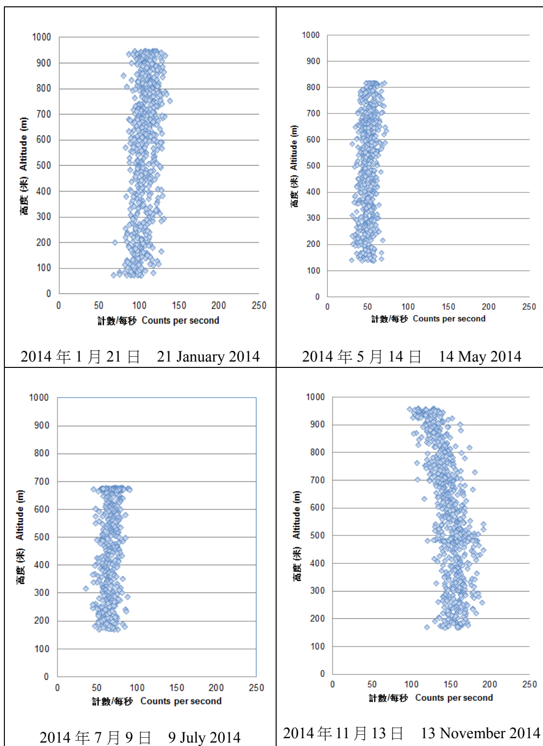
圖 4. 空中輻射監測系統在二零一四年於大鵬灣海面上空測量到的計數率隨高度的變化。 Figure 4. Variation of count rate with altitude at Mirs Bay, as measured by the Aerial Radiation Monitoring System in 2014.
