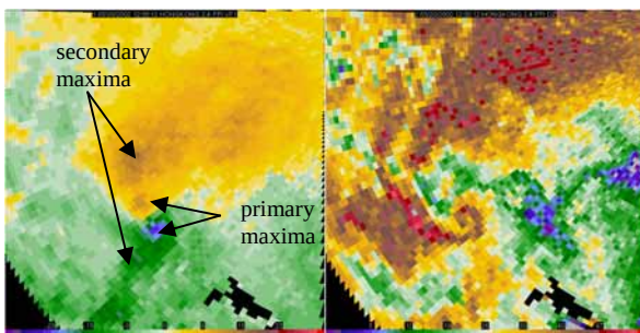
FIG. 1: Radial velocity (left) and reflectivity (right) plot of TDWR observation of the tornado at 12:30 UTC, 20 May 2002.
