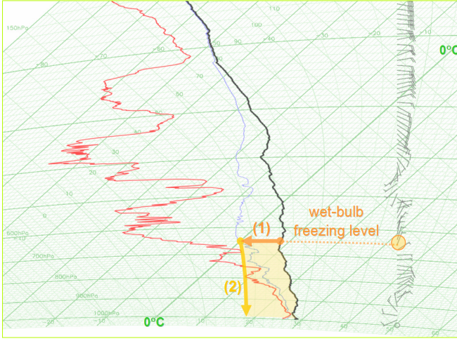
Fig. 2 Two-stage thermodynamic processes of downdraft — (1) isobaric cooling by evaporation of raindrops; (2) pseudo-adiabatic descent if favourable (i.e. inequality (2) satisfied). The shaded area represents DCAPE and is positive (negatively buoyant) in this illustration. The black, blue and red traces on the tephigram represent dry-bulb, wet-bulb and dew-point temperatures respectively.
