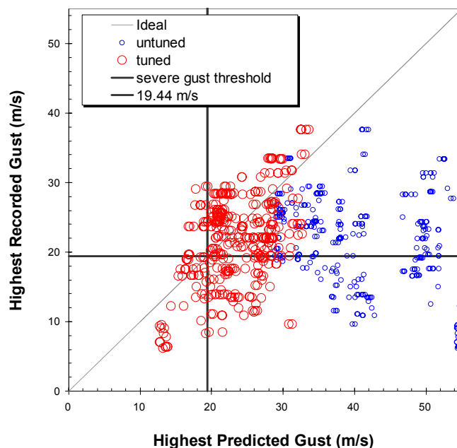
Fig. 5 Scatter plot showing highest recorded gust versus the predicted maximum convective gust in the test data set. Blue and red circles represent respectively predictions before and after tuning.
