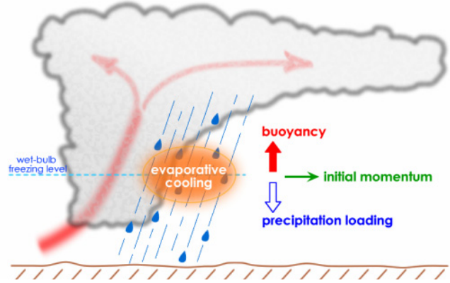
Fig. 1 Schematic diagram illustrating the conceptual model of convective downdraft due to raindrops evaporative cooling of air parcel in the rain shaft.
