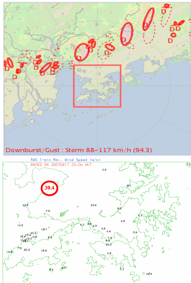
Fig. 4 Squall line on 17 April 2007. Upper panel shows the first severe downburst/squalls alert message (94.3 km/h or 26.7 m/s) issued at 7:24 pm. (Plot convention: red ellipses tagged with letter "D" represent downburst/squalls threat areas; dashed ellipses represent forecast positions at 30 min lead time; warning zone of Hong Kong is bounded by red lines. Also shown on the background is the map of Hong Kong and neighbouring regions, overlaid with 3-km reflectivity map.) Lower panel displays the 1-min maximum wind speed (i.e. the maximum of sixty 1-sec wind gust records) at 8:06 pm when severe gust (30.4 m/s) was first detected in Hong Kong at the AWS encircled in red.
