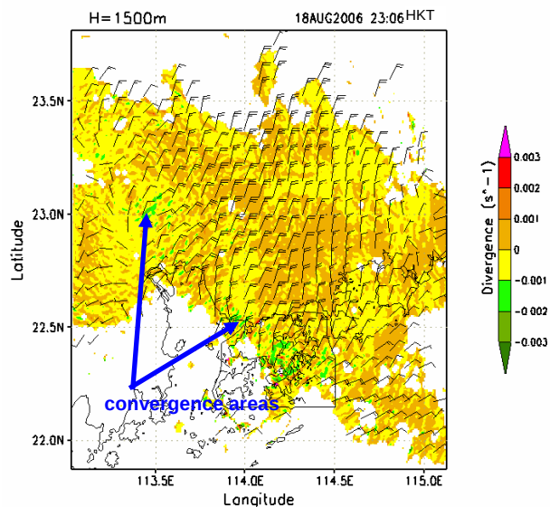
Figure 11 Divergence field at 1500 m AMSL at 23:06 HKT, 18 August 2006.
