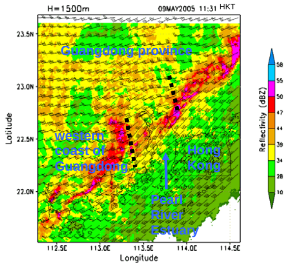
Figure 1 Radar reflectivity and horizontal wind vector at 1500 m AMSL at 11:31 HKT, 9 May 2005. Axes of westerly waves are indicated by broken lines
