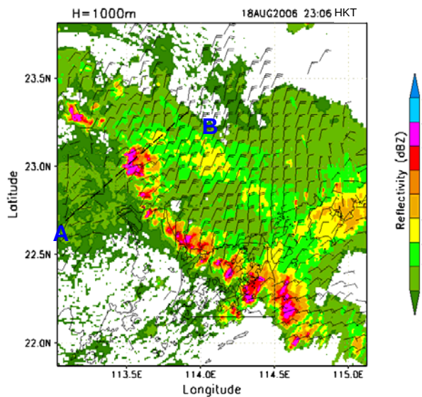
Figure 9 Radar reflectivity and horizontal wind vector at 1000 m AMSL at 23:06 HKT, 18 August 2006.
