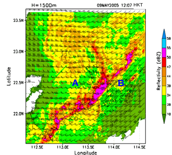
Figure 4 Radar reflectivity and horizontal wind vector at 1500 m AMSL at 12:07 HKT, 9 May 2005.
