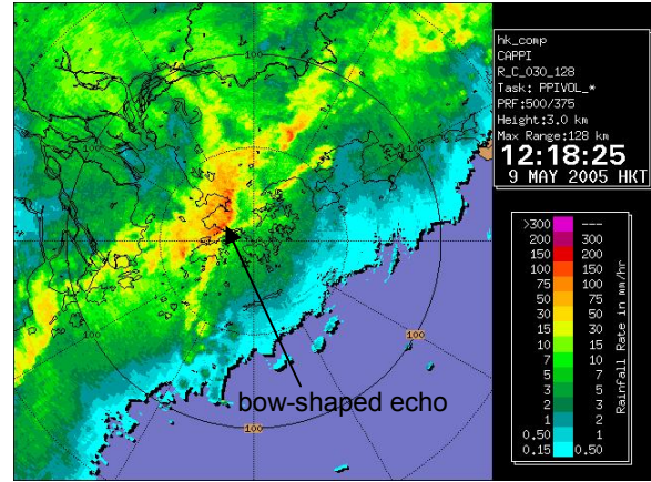
Figure 2 128-km range radar picture of Hong Kong at 12:18 p.m., 9 May 2005, showing the passage of the squall line across the territory.
