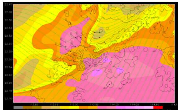
Figure 10 The simulated surface wind magnitude (colour shaded), streamlines (green lines) and winds at the anemometer locations (wind barbs) at 12:50 p.m., 9 May 2005.
