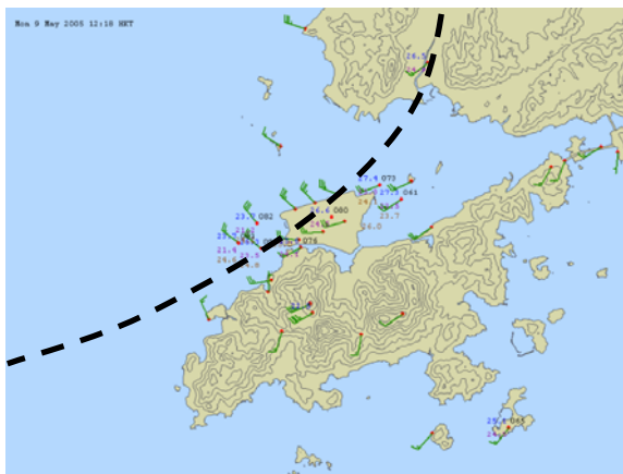
Figure 3 Surface observations at 12:18 p.m., 9 May 2005, with the estimated location of the squall line indicated by a dashed line.
