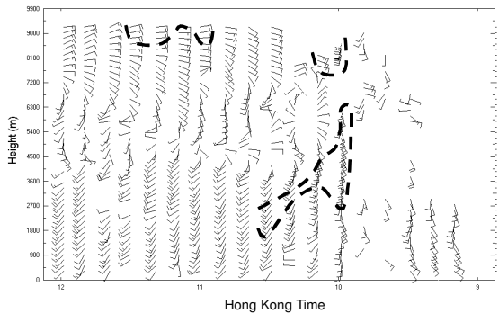
Figure 10 Sham Shui Po wind profiler data between 9 a.m. and noon of 14 September 2002. The major jets of more than 20 knots are indicated by broken lines.
