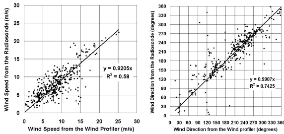
Figure 1 Comparison between Sham Shui Po wind profiler and King's Park radiosonde for wind speed (left) and direction (right).
