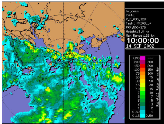
Figure 9 Weather radar imagery at 10 a.m., 14 September 2002.
