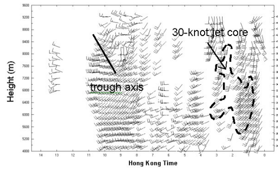
Figure 7 Sham Shui Po wind profiler data between midnight and 2 p.m. of 17 July 2002 (only data above 4.8 km are shown).
