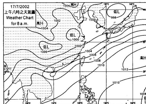
Figure 3 Surface weather chart at 8 a.m., 17 July 2002.
