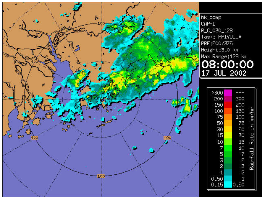
Figure 5 Weather radar imagery at 8 a.m., 17 July 2002.
