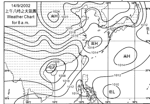
Figure 8 Surface weather chart at 8 a.m., 14 September 2002.
