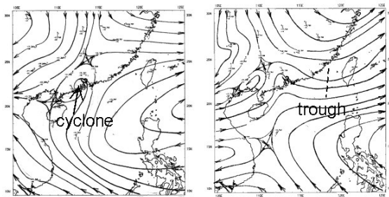
Figure 6 Streamline analyses of 400-hPa winds at 8 a.m. (left) and 8 p.m. (right) of 17 July 2002.
