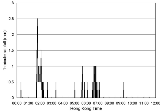
Figure 4 Time-series of 1-minute rainfall at King's Park in the morning of 17 July 2002.
