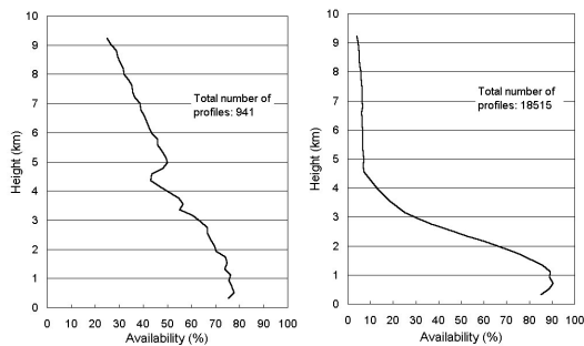
Figure 2 Data availability at different levels of Sham Shui Po wind profiler in rain (left) and no rain (right) conditions.
