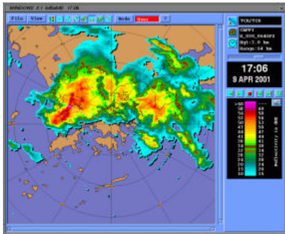
(a) 3-km CAPPI reflectivity at 5:06 p.m.
