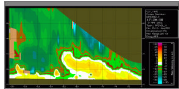
Fig. 6 - Doppler vertical section along an E-W radial segment (looking north, i.e. radar on the right; horizontal distance and altitude at 2-km interval). Maximum velocity away from radar (solid arrow) at 3-km level 10 km from radar was around 10 \text{ m s}^{-1} ; maximum velocity towards radar (dashed arrow) was around 30 \text{ m s}^{-1} about 3 to 4 km high and 15 km from radar.
