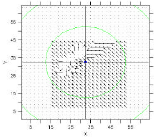
(a) Grid winds input at 1-km level
