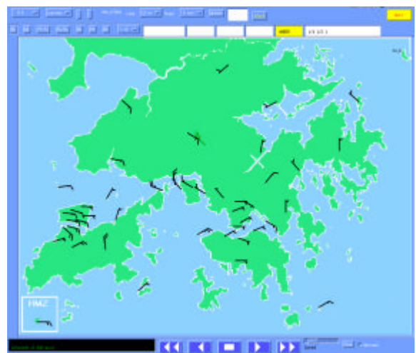
Fig. 4 - AWS winds at 5:30 p.m., with the pair of convergence (solid) and divergence (dashed) lines as implied from the streamline analysis.
