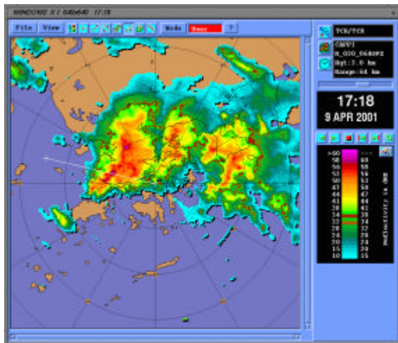
(c) 3-km CAPPI reflectivity at 5:18 p.m.
