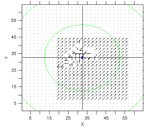
(b) Grid winds input at 3-km level
