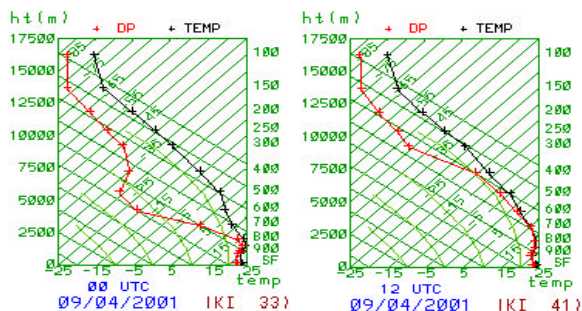
Fig. 2 - Tephigrams from ORSM analyses at 00 UTC (left) and 12 UTC (right) on 9 April 2001, showing a significant moistening of the mid-troposphere after the passage of the hailstorm.
