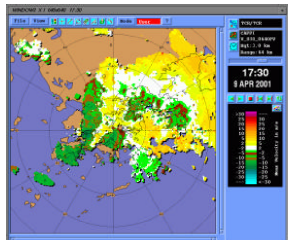
(f) 3-km level Doppler maps at 5:30 p.m.
