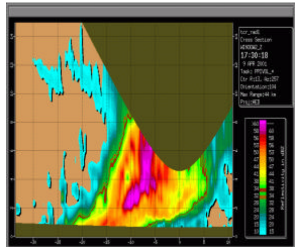
(f) Vertical section along X - Y for (e)
