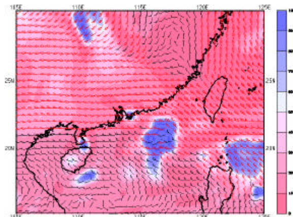
Fig. 3 - ORSM 8-hour forecast of 500-hPa wind and relative humidity fields, valid at 4 p.m. on 9 April 2001. A moist pocket was forecast to develop right over Hong Kong. In reality, the extent of moistening in the mid-troposphere was even more widespread and persistent.
