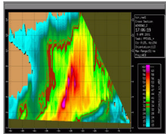
(b) Vertical section along X - Y for (a)
