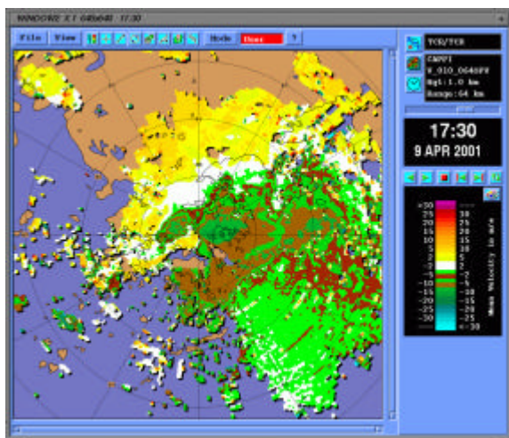
(e) 1-km level Doppler maps at 5:30 p.m.
