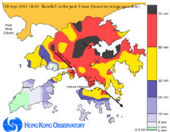
Fig. 1 - Rainfall (mm) distribution between 3 p.m. and 6 p.m. on 9 April 2001, with heavy dots showing the trail of hailstone reports spreading southeastwards across Hong Kong between 5:35 p.m. and 5:50 p.m. that day.
