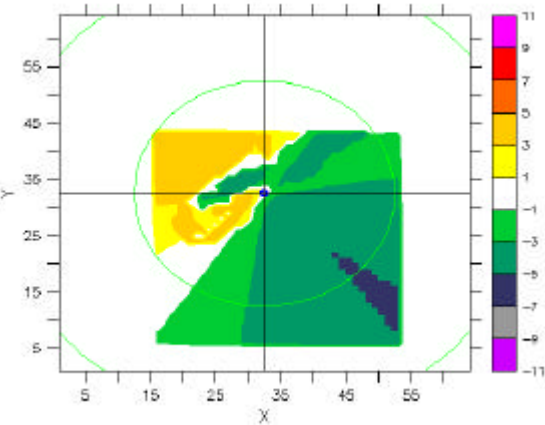
(c) 1-km level computed Doppler field
