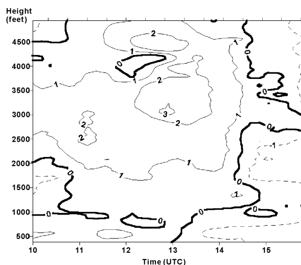
Figure 7 Vertical winds detected by Sha Lo Wan profiler between 10-15Z 8 March 1999. Updraughts (in \text{ms}^{-1} ) are positive.
