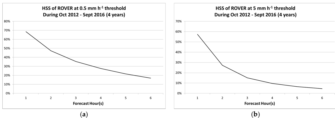
Figure 12. HSS of ROVER at: (a) 0.5 mm·h -1 ; and (b) mm·h -1 thresholds based on four years of data.
