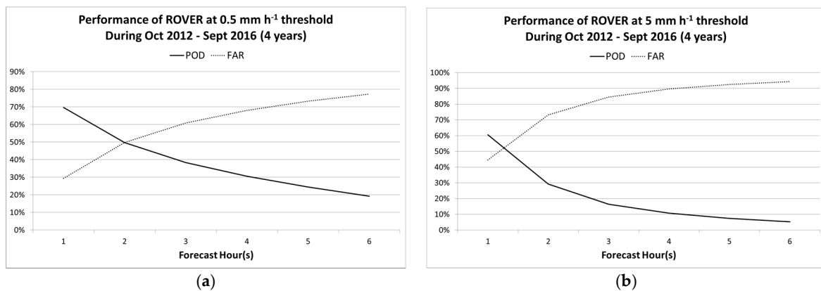
Figure 11. POD and FAR of ROVER at: (a) 0.5 mm·h -1 ; and (b) 5 mm·h -1 thresholds based on four years of data.
