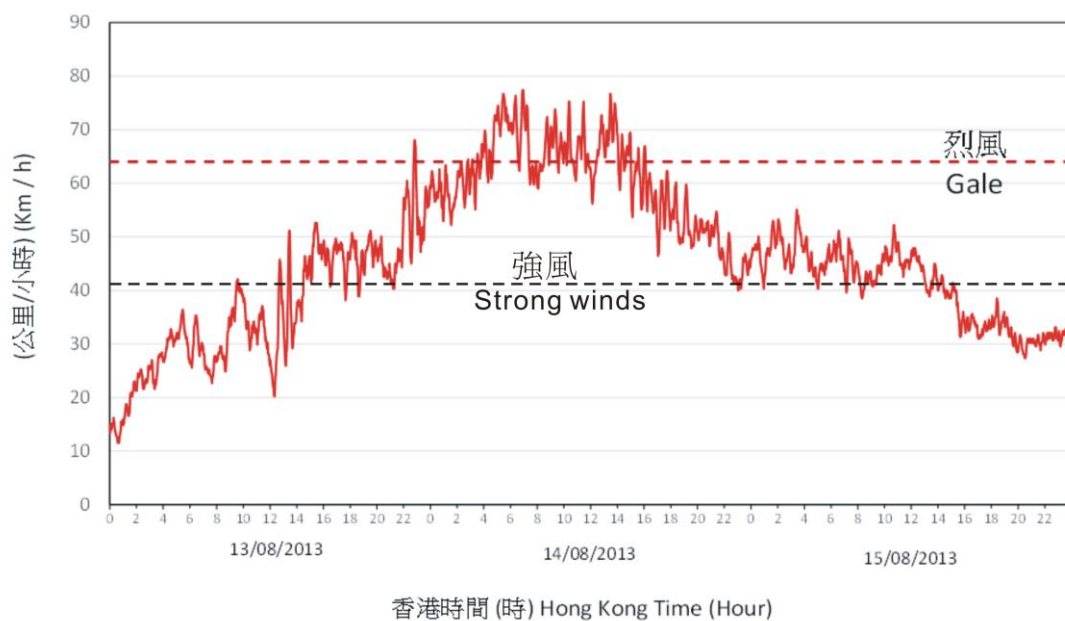
圖 3.5.4a 二零一三年八月十三日至十五日長洲自動氣象站錄得的十分鐘平均風速。 Figure 3.5.4a Trace of 10-minute mean wind speed recorded at Cheung Chau automatic weather station on 13 - 15 August 2013.
