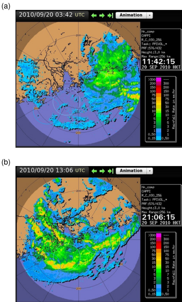
Fig. 3 Samples of radar imagery showing the convection severity relating to (a) Yellow for the holding area ABBEY, and (b) Red for all the three key holding areas ABBEY, CANTO and GAMBA as marked by circles in Fig. 2..
