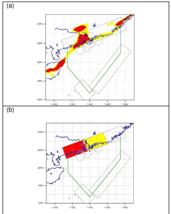
Fig. 4 Significant convection forecast for the next 3 hours (red and yellow indicate high and medium chance over the coloured regions respectively). The presentation in (a) mimics the convective weather pattern while (b) shows the overall chance of significant convection within each boxed or circled area.
