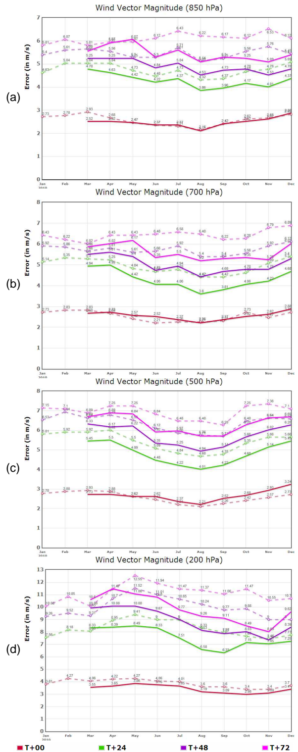
Fig. 4. RMSE of analysis and forecast of wind vectors from Meso-NHM (solid lines) and ORSM (dotted lines) during Mar-Dec 2010 on (a) 850 hPa, (b) 700 hPa, (c) 500 hPa and (d) 200 hPa.
