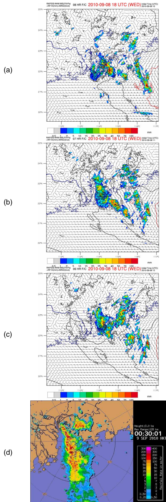
Fig. 7. RAPIDS-NHM forecasts of hourly accumulated rainfall and mean-sea-level pressure at 02:00 HKT 9 September 2010, with model runs initialized from 10 to 12 UTC 8 September shown in (a)-(c) respectively; radar reflectivity image at 00:30 HKT 9 September 2010 shown in (d)
